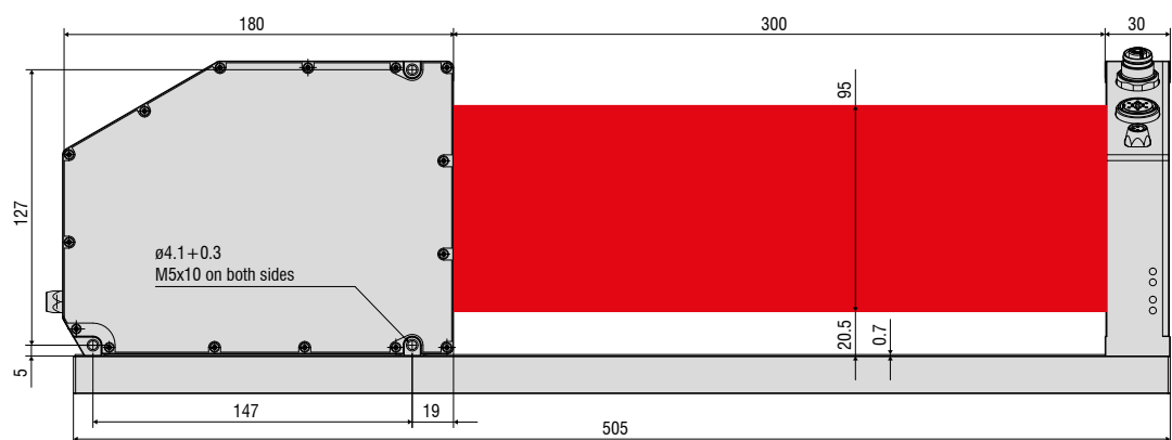
Light source
